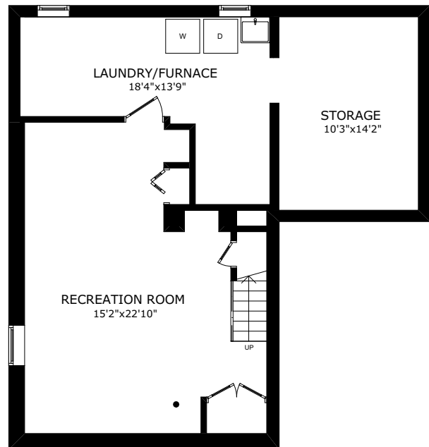
BASEMENT
